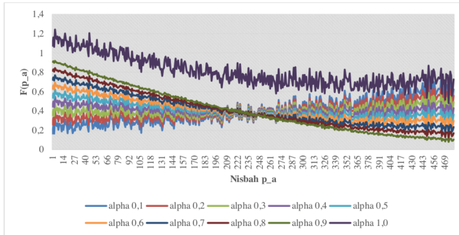
Figure 2. Plot of Objective Function F(p_a) for all values of \alpha
